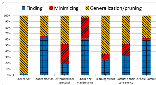
Figure 3. Runtime break down for each of the seven protocols we verified using I4.
